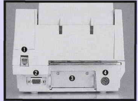
① Cash Drawer Support(6 pin Modular) ② Standard RS-232C Interface(D-Sub 9 pin) ③ Optional Interface Slot ④ Power Supply Connector
